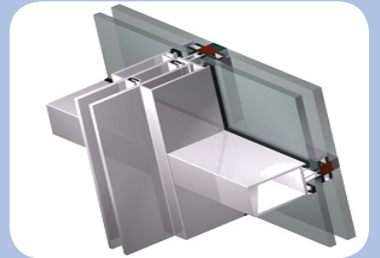
↑ Securing aluminium curtain walling
