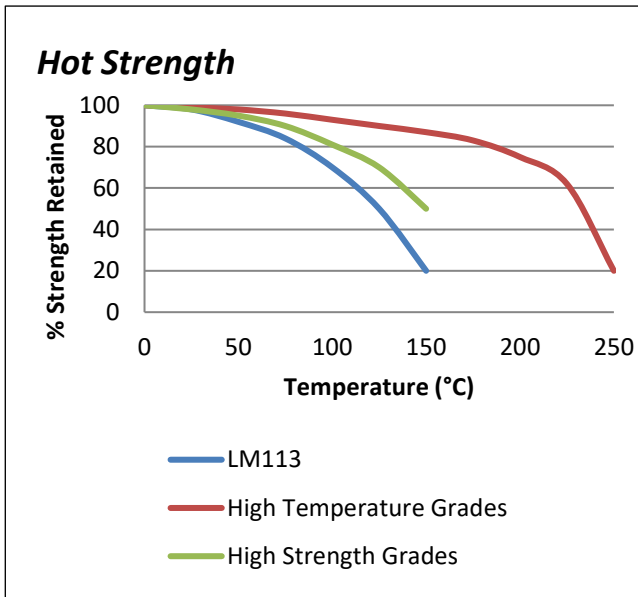
"Hot strength" Breakaway strength on M10 Zinc plated bolts according to ISO 10964. Cured at 23°C for 24 hours then conditioned for 30 minutes at testing temperature.
